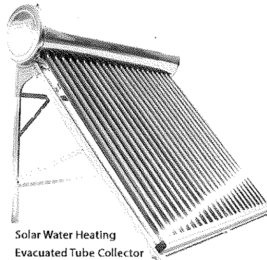
Figure 5. Solar Evacuated Water Heater
