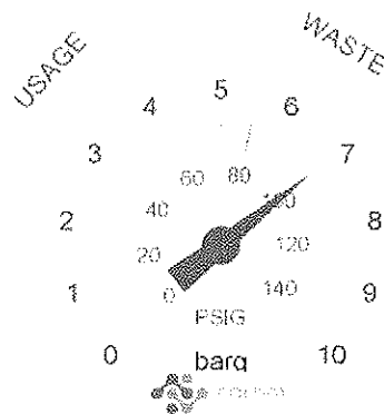
Figure 4. Artificial Demand of Air Compressor
