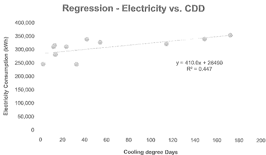
Figure 2. Regression – Electricity vs. CDD
