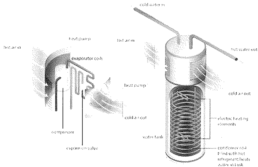
Figure 6. Heat Pump
