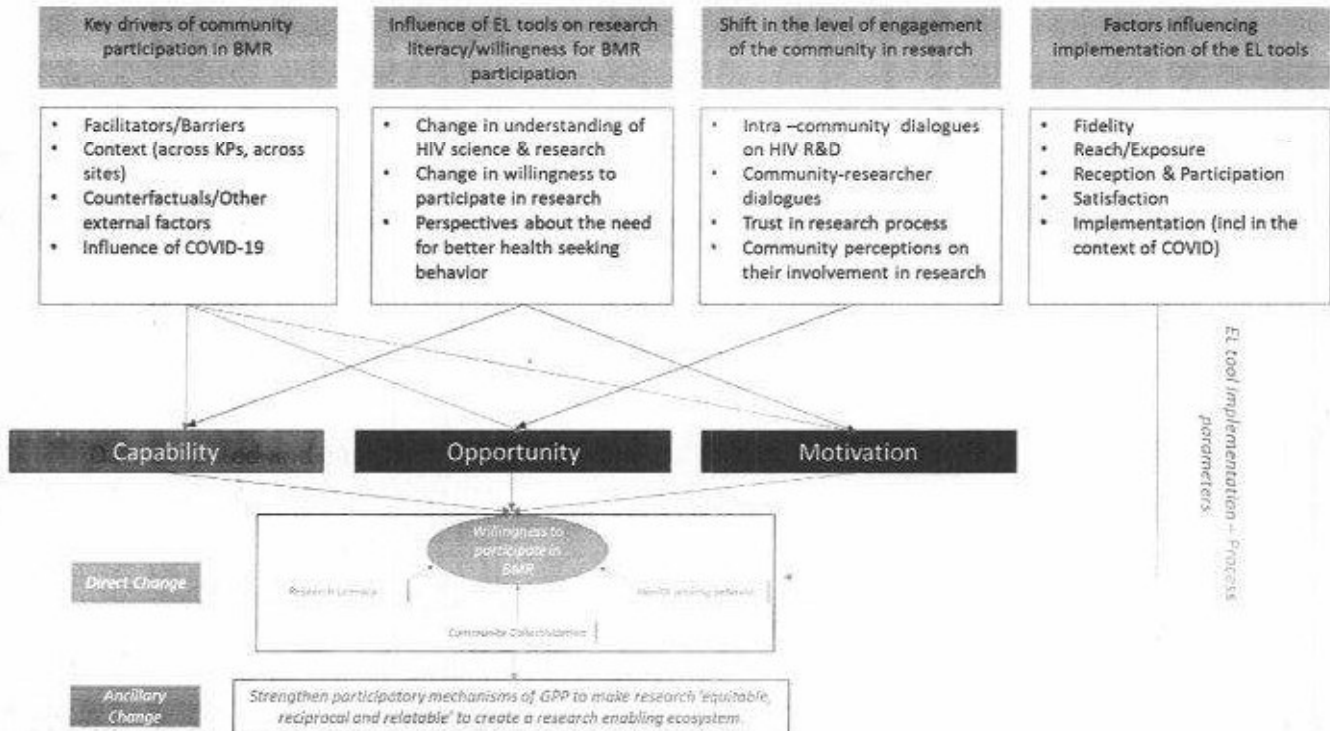
Figure 6: Study Outcomes
